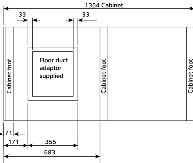
600/900 horizontal versions
