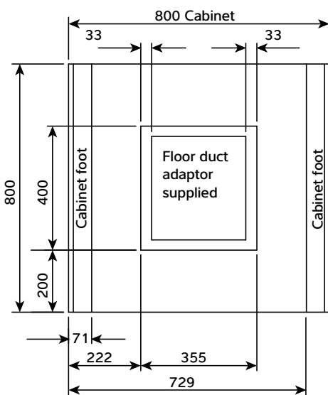
1200/1500 vertical versions
