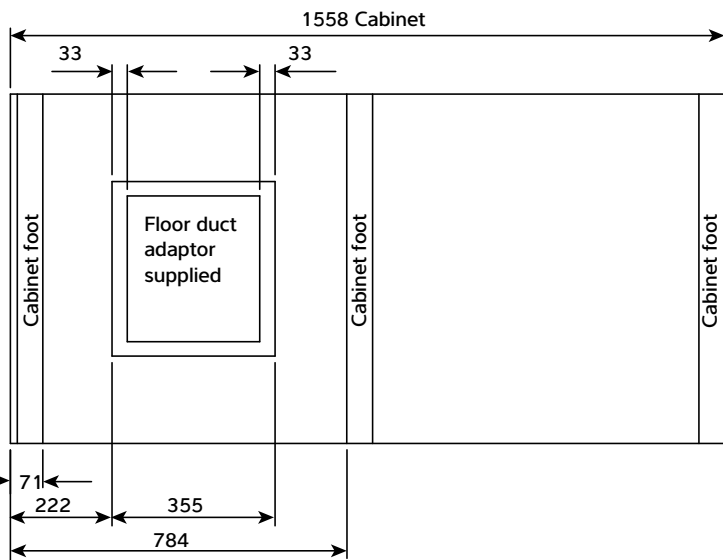
1200/1500 horizontal versions
