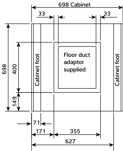
600/900 vertical versions
